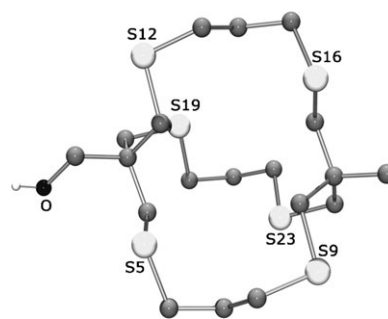
Fig. 2 Structure of 11 (one of two independent molecules is shown). Details about bond lengths and angles are contained in Table S2 of the ESI†.
