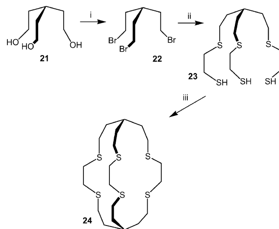
Scheme 4 Synthesis of the cage 24 : (i) \text{PBr}_3-\text{HBr} ; (ii) \text{HS}(\text{CH}_2)_2-\text{SH} , \text{EtONa} in \text{EtOH} ; (iii) 22 , \text{Cs}_2\text{CO}_3 in \text{DMF} .
