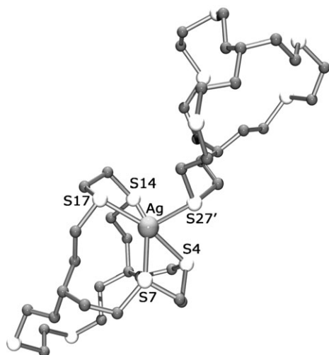
Fig. 5 Structure of the complex cation of [Ag( 24 )]triflate. Selected bond lengths and angles: Ag–S4 2.603(3), Ag–S7 2.800(3), Ag–S14 2.967(3), Ag–S17 2.516(3), Ag–S27' 2.687(3) Å; S4–Ag–S7 81.21(10), S4–Ag–S14 91.61(10), S4–Ag–S17 163.37(10), S4–Ag–S27' 88.36(9), S7–Ag–S14 150.18(9), S7–Ag–S17 98.39(10), S7–Ag–S27' 88.43(8), S14–Ag–S17 80.48(11), S14–Ag–S27' 120.45(9), S17–Ag–S27' 108.26(9) (Symmetry operation: -x + 3/2, -y, z + 1/2 ).
