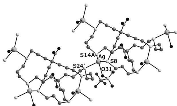
Fig. 4 Structure of the complex cation of [\text{Ag}(\mathbf{18})]\text{triflate} . Sulfur atom S14 is disordered over two sites. S14A represents the major site with occupancy of 0.915 and S14B with 0.085 occupancy. The minor site is not shown for clarity. Selected bond lengths: \text{Ag}-\text{O31} 2.526(4), \text{Ag}-\text{S8} 2.5164(15), \text{Ag}-\text{S14A} 2.5090(16), \text{Ag}-\text{S24}' 2.6231(15). (Symmetry operation: -x + 1/2, y - 1/2, -z + 1/2 ).
