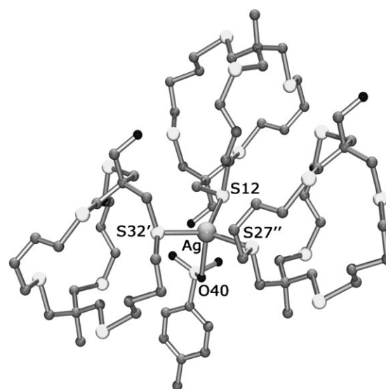
Fig. 3 Structure of the complex cation of [Ag(14)] tosylate. Selected bond lengths and angles: Ag–S12 2.563(4), Ag–O40 2.438(8), Ag–S32' 2.511(4), Ag–S27'' 2.552(4) Å; S12–Ag–O40 106.3(2) , S12–Ag–S32' 122.64(13) , S12–Ag–S27'' 104.07(13)^\circ (Symmetry operations: (') 1-x, -y, -z ; (') -x, -y, -z ).
