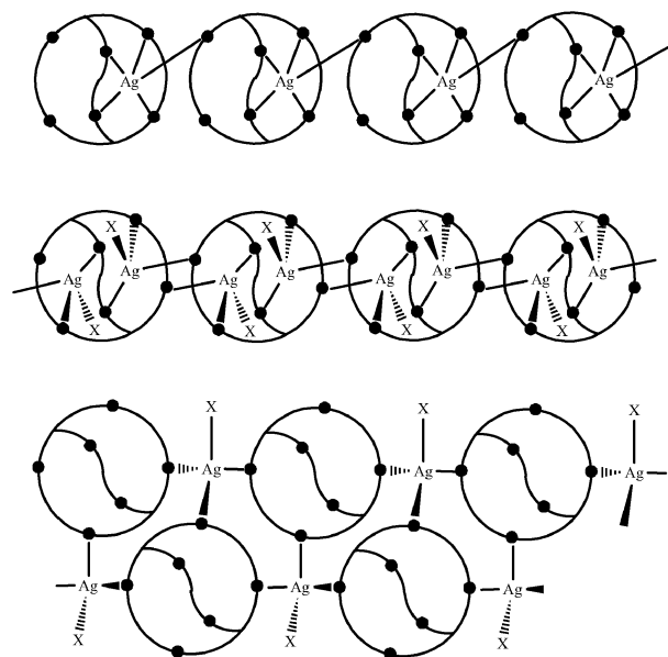
Fig. 6 Schematic view of the coordination modes of several \text{S}_6 -cages. Black dots represent thioether sulfur atoms and X the counter ions. Top: [Ag( 24 )]triflate; Middle: [Ag( 18 )]triflate; Bottom: [Ag( 14 )]tosylate.
