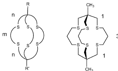
Scheme 1 Basic structure of the S 6 -cages, abbreviated as R,R' -[nmn-S 6 ] (left) and as an example CH 3 CH 3 -[131-S 6 ] (right).
