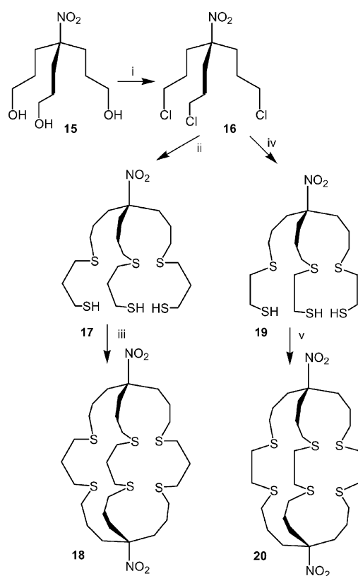
Scheme 3 Synthesis of the cages 18 and 20 : (i) \text{SO}_2\text{Cl}_2 ; (ii) \text{HS}-(\text{CH}_2)_3-\text{SH} , \text{EtONa} in \text{EtOH} ; (iii) 16 , \text{Cs}_2\text{CO}_3 in \text{DMF} ; (iv) \text{HS}(\text{CH}_2)_2-\text{SH} , \text{EtONa} in \text{EtOH} ; (v) 16 , \text{Cs}_2\text{CO}_3 in \text{DMF} .
