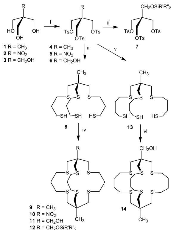
Scheme 2 Synthesis of the cages 9–12 and 14 : (i) TsCl in pyridine; (ii) tert -butyldimethyl-silyl chloride, imidazole in DMF; (iii) HS-(CH 2 ) 3 -SH, EtONa in EtOH; (iv) 4–7 , Cs 2 CO 3 in DMF; (v) HS-(CH 2 ) 4 -SH, EtONa in EtOH; (vi) 6 , Cs 2 CO 3 in DMF.
