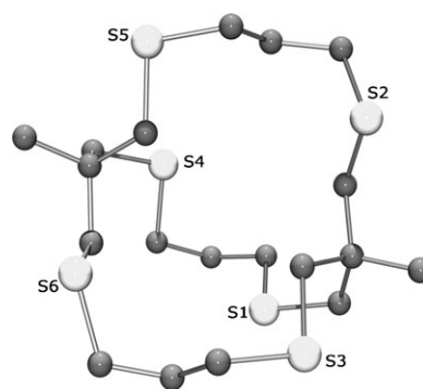
Fig. 1 Structure of 9 with the exo orientation of the lone pairs of the thioether sulfur atoms. Details about bond lengths and angles are contained in Table S1 of the ESI†.
